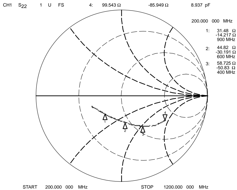
Figure 3. LNA Input and Output Match (at Device Pin)
